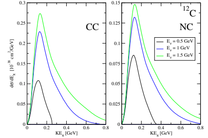
Figure 5: Differential cross section versus pion kinetic energy.
