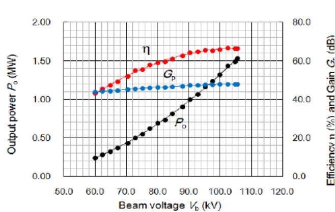
Measured data (no mismatch used at the output) Courtesy of Toshiba
