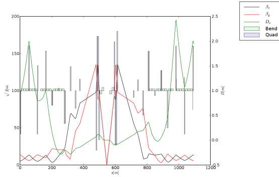
Figure 2: Beam 1 collision optics for the dipole first layout. The boxes in blue represent the quadrupoles and their height is proportional to the gradient. The green boxed represent the bending magnets and their height is proportional to the bending field.
