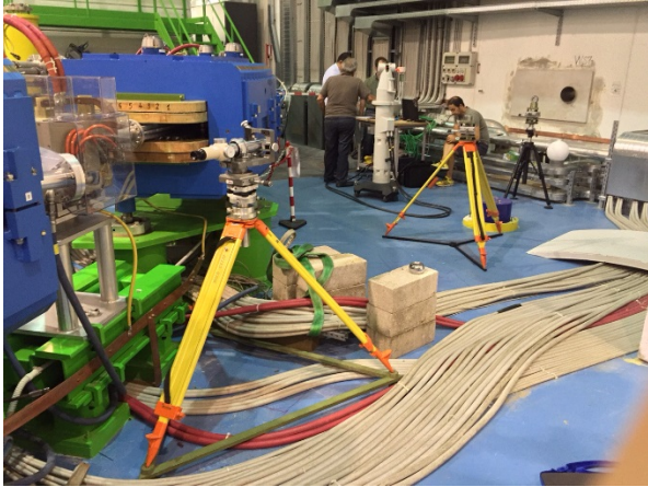
Figure 4: Step 3 (setting the telescope linesight through P2 and P3)
