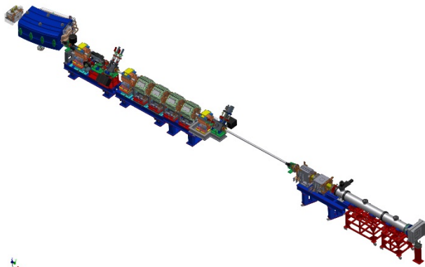
Figure 3: The new XPR line in a preliminary design (now changed). At the big dipole (left) start the line; the nude pipe in the middle crosses the wall.
