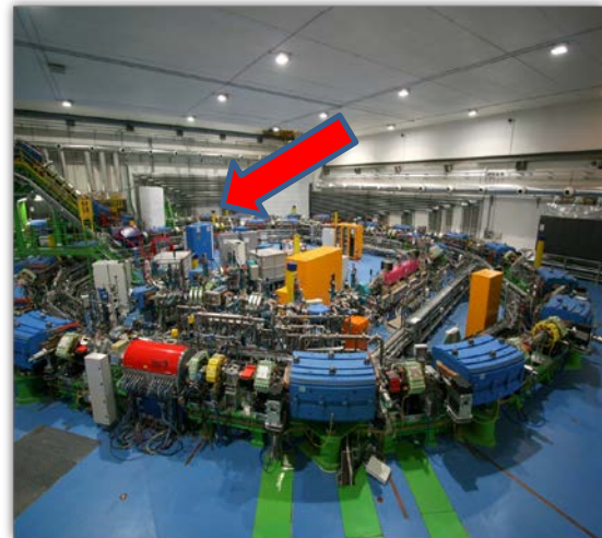
Figure 1: The Accelerator Hall and the hole towards the XPR Hall
