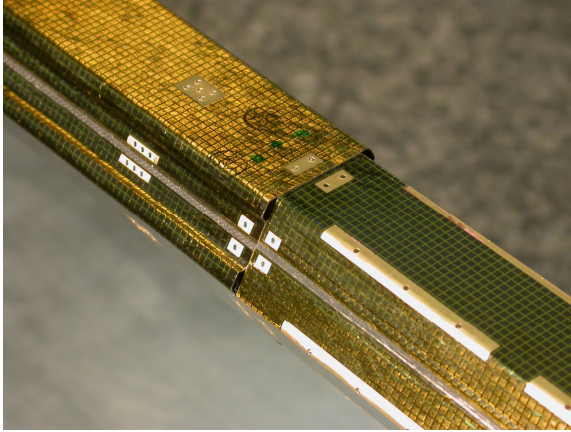
Fig. 9. Copper mesh co cured onto the carbon fiber mechanical support.
