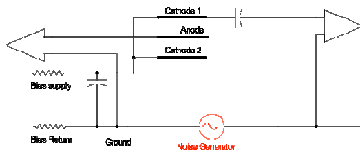
Fig. 8. This is identical to fig. 7 but the gap in the ground plane replaced by a noise generator. The gap was shorted together but the difference in potentials between the two grounds causes current to flow through the ground plane. The resistance in this connection causes a noise voltage.
