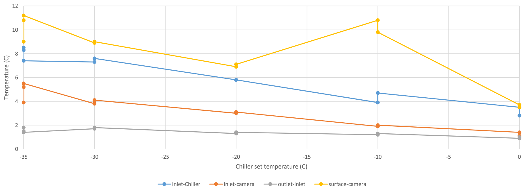
Aluminum block Temperature differences among sensors
