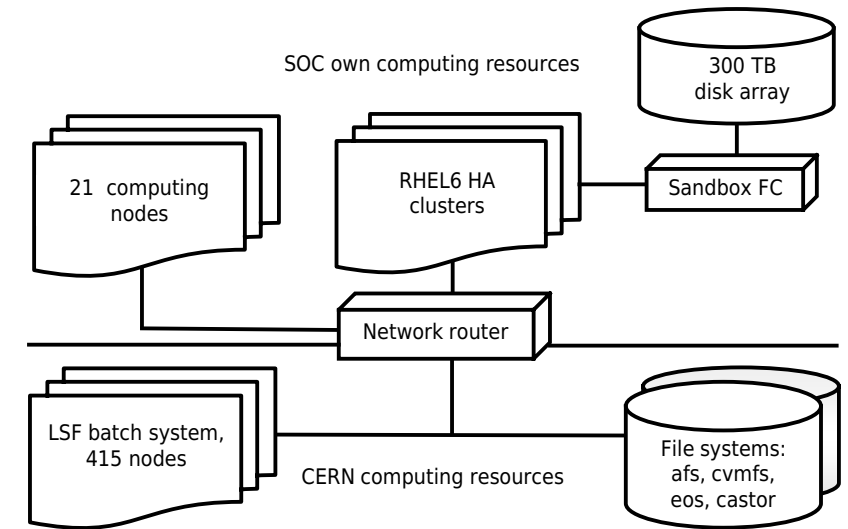
Figure 1. SOC infrastructure
