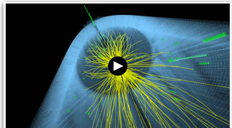
Higgs boson candidate event from 2012 data (8 TeV) recorded by the CMS experiment: ZZ to four electrons
