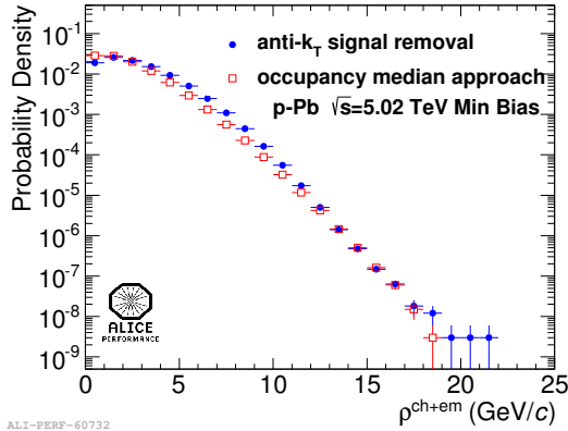
Figure 1. The probability density for extracting a certain momentum area density \rho_{full}^{BKG,corr.} (labeled as \rho^{ch+em} ), which describes the background of charged and neutral signals to the measured jet p_T in the event. The method described in the text is labeled “occupancy median approach”. Another approach, not further discussed here, is the exclusion of overlap between a anti- k_T signal jet and a k_T background jet (blue dots).
