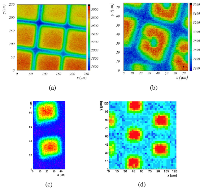
Figure 1: Two-dimensional scans for (a) Hamamatsu H100C, (b) CPTA/Photonique and (c) & (d) STMicronics. Surface scans are valuable to assess the surface sensitivity of SiPMs, (a),(b) & (c) were performed with a step size of 1 \mu\text{m} and clearly show the structure of individual SiPM cells. (d) shows a part of a larger surface scan (STMicronics with a step size of 3 \mu\text{m} ).
