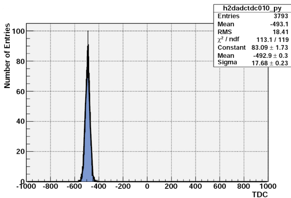
Figure 5: Timing resolution for back-to-back \gamma 's ( 25 \text{ ps/bin} \rightarrow \sigma_t \sim 442 \text{ ps} ). Hamamatsu 3 \times 3 \text{ mm}^2 SiPMs were used for this measurement.
