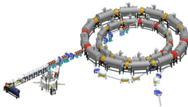
FFAG Accelerators
