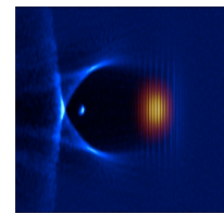
Laser Plasma Accelerators
