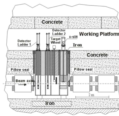
Figure 2.4-126 Schematic layout of the target area of the Super-FRS. A vertical plug system has been adapted which has proven to guarantee a safe and reliable operation at PSI in a very high radiation field. Routine maintenance at PSI is done about once per year.
