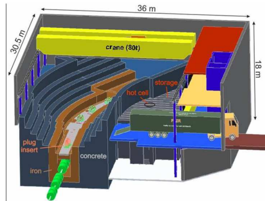
Figure 2.4-175 Layout of the Super-FRS target building. The top part of the concrete shielding can be removed to access the working platform. Heavy devices can be transported by crane to the nearby hot cell, storage places or directly onto a truck which can drive into the hall.
