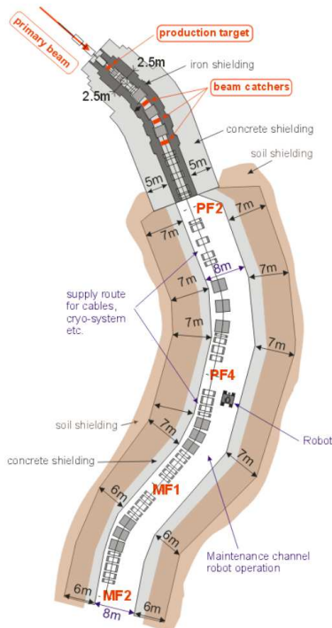
Figure 2.4-166 Schematic layout of the Super-FRS with beam line and shielding measures. The area from the target up to the intermediate focal plane PF2 of the Pre-Separator is shielded with iron in order to provide a compact radiation protection in the target building. The concrete in the Main-Separator can be partially replaced by soil taking into account an about 20% smaller absorption of the soil.
