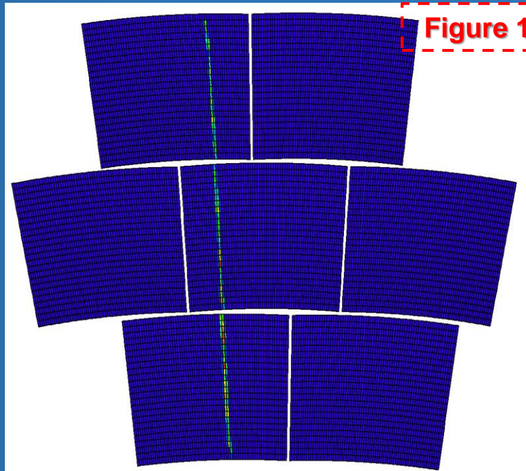
Micromegas modules on the LTPC endplate .
