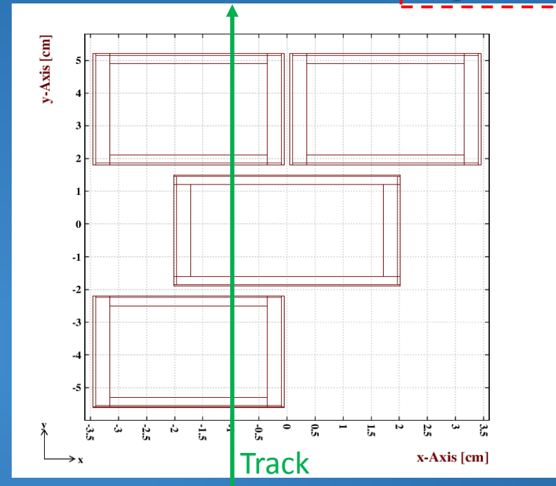
The simulated Micromegas modules
