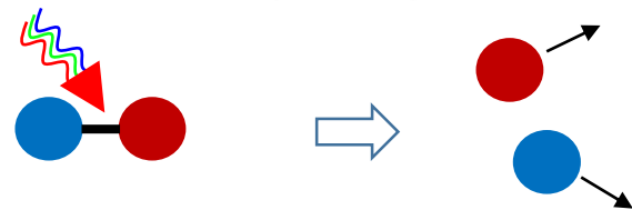
Molecular break-up using laser beam
