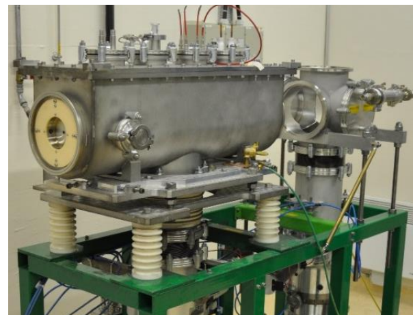
RFQ cooler
