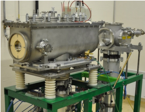
RFQ cooler
