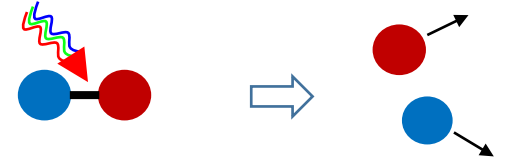
Molecular break-up using laser beam
