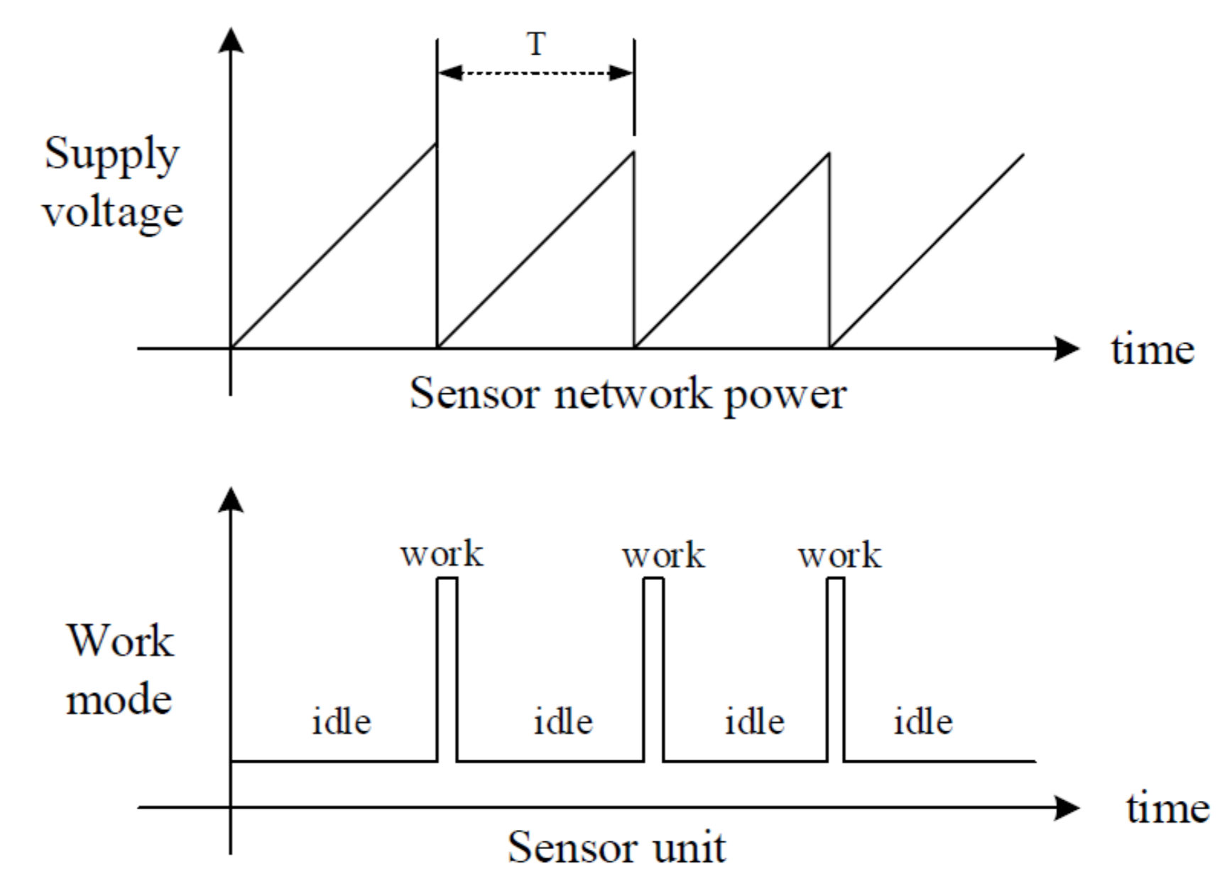
Fig.5 Saw wave voltage power supplier
