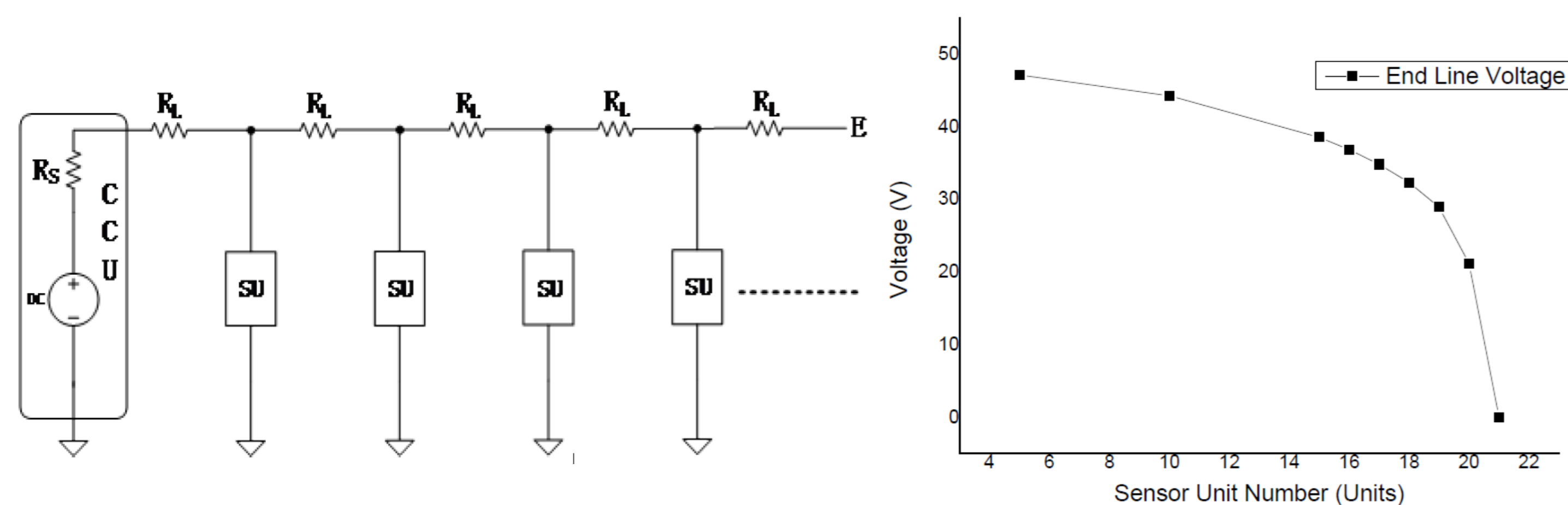
Fig.2 Power line model for fig.1
