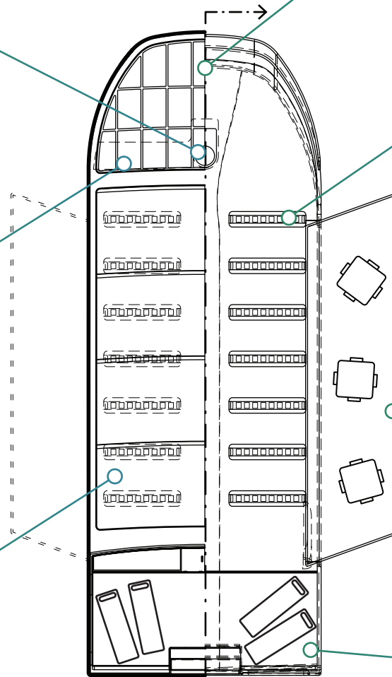
TOP / CROSS SECTION HYDROPIA "Whale"
