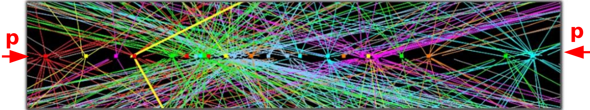
Atlas event with a Z boson decaying to two muons and 24 additional interaction vertices.
