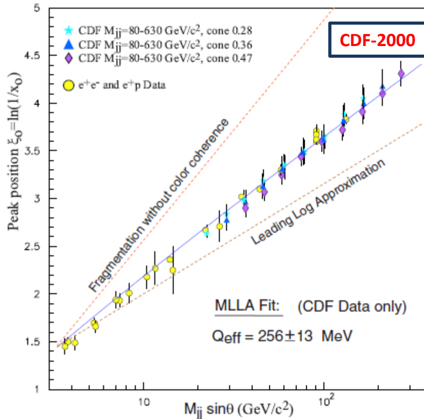
Figure 2. Peak position \xi^* of the inclusive \xi distribution plotted against di-jet mass \times \sin\Theta_0 in comparison with the MLLA prediction (central curve); also shown are (in arbitrary normalization) the double logarithmic approximation (lower curve with asymptotic slope \xi^* \sim Y/2 ) and expectation from cascade without coherence. Result by CDF Collaboration | (2000)
