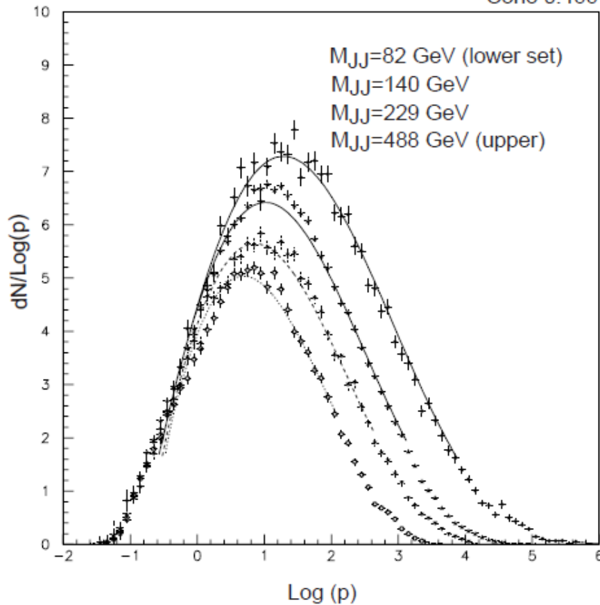
dN/d\log(p) distribution (4 dijet mass samples, cone 0.466).
