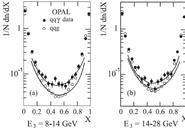
Fig. 1.3 Charged particle flow in between the two quark jets of the q\bar{q}g and q\bar{q}\gamma final states, as measured by OPAL [62], for two samples of energies E_3 of the lowest energy
