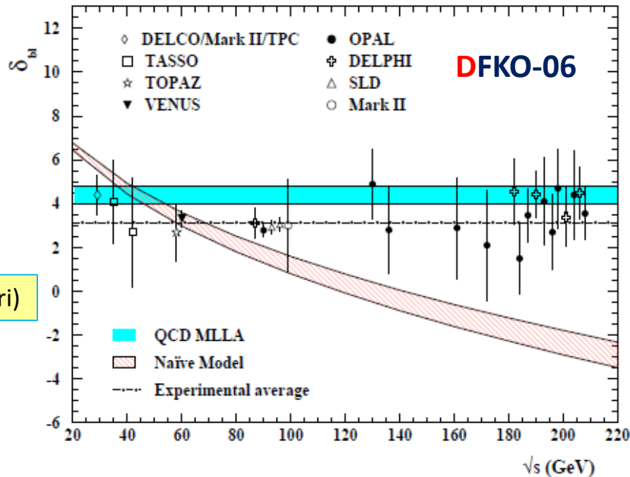
Figure 2: Experimental measurements of \delta_{bc} plotted as a function of the c.m.s. energy, \sqrt{s} ; data below 90 GeV reevaluated (see Appendix B.2). The revised MLLA expectation using \delta_{bc}^{MLLA} = 4.4 \pm 0.4 is indicated by the shaded area. Also shown is the “naïve model” [16] based on the reduction of energy scale (dashed area).
