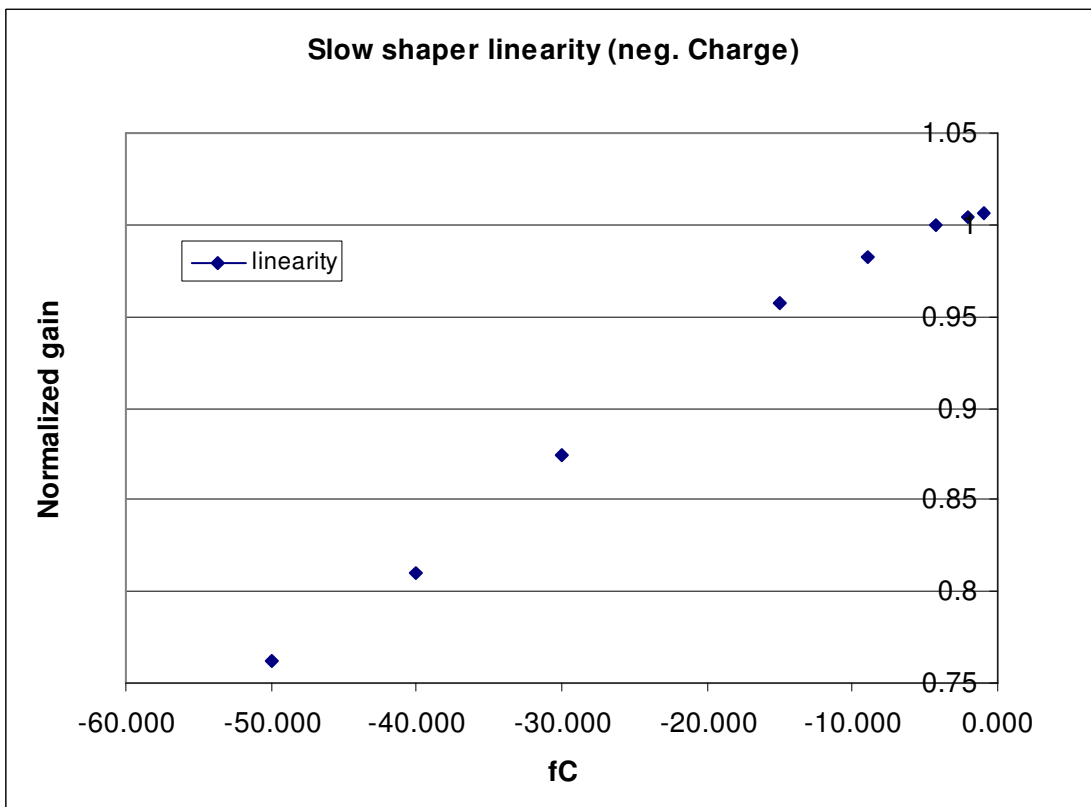
Nonlinearity for the slow shaper, for positive and negative charges.
