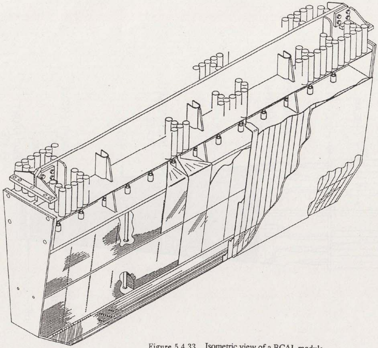
Figure 5.4.33 Isometric view of a BCAL module.
