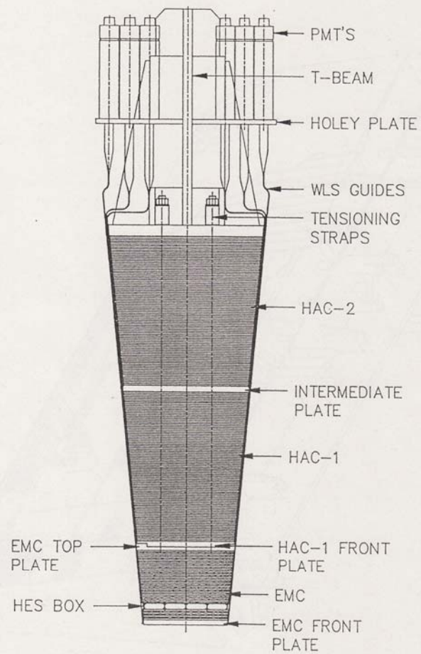
Figure 5.4.34 Transverse cross section through a BCAL module showing the structural elements.
