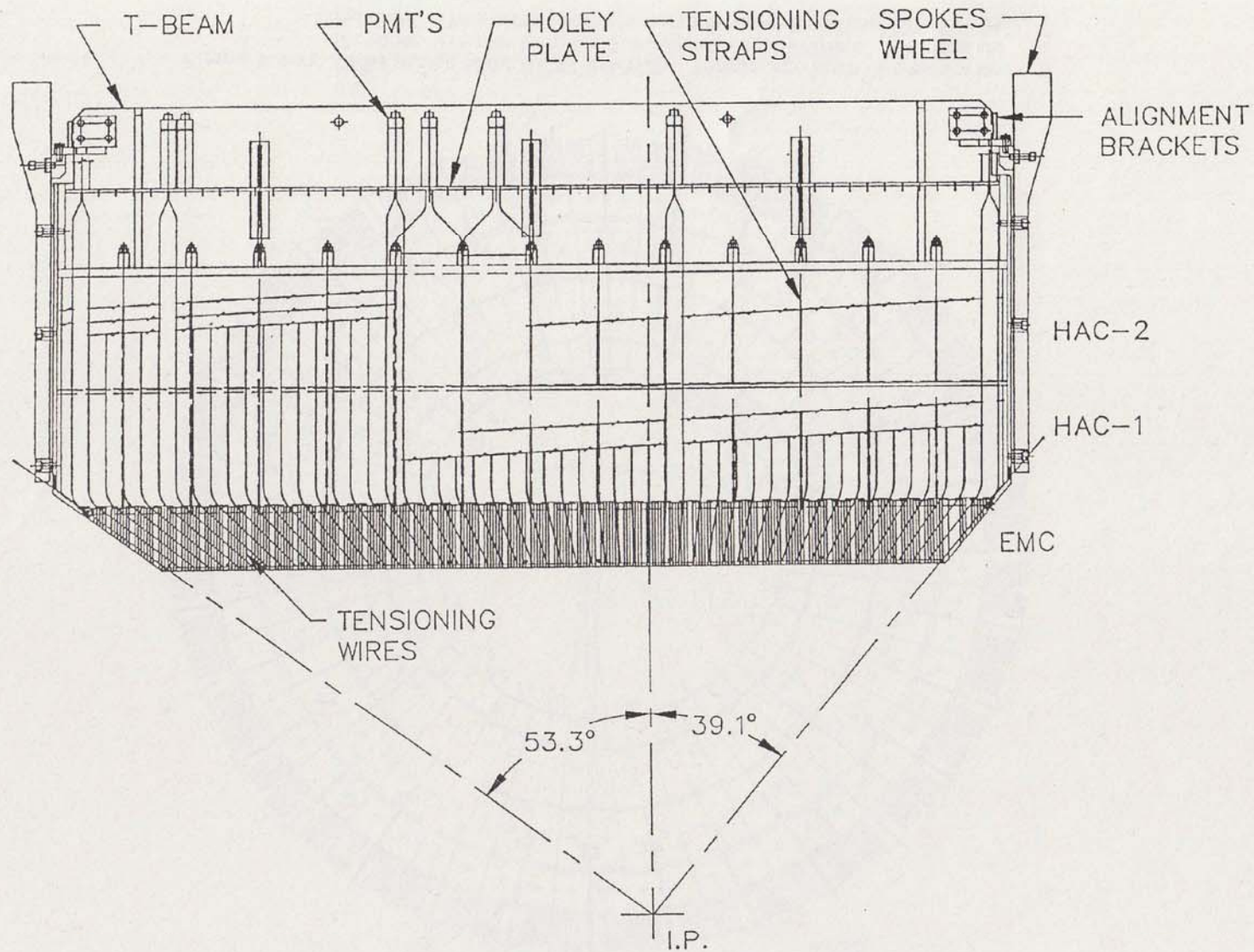
Figure 5.4.32 Longitudinal cross section of a BCAL module.
