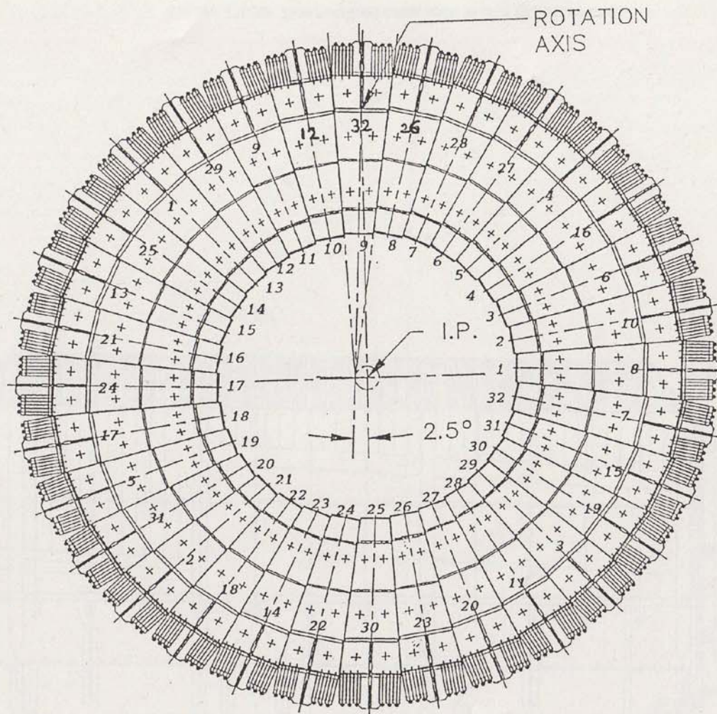
Figure 5.4.31 Cross section of the BCAL assembly. The electron beam direction is into the paper. The number of modules loaded into the different locations are indicated. The numbers at the inner radius show the official ZEUS BCAL numbering scheme.
