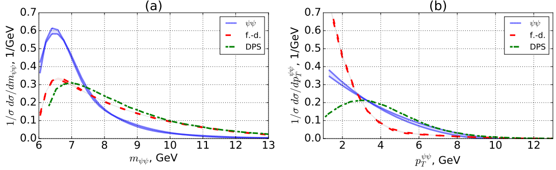
Figure 4. Distributions over invariant mass (left panel) and transverse momentum (right panel) of the charmonium pair
