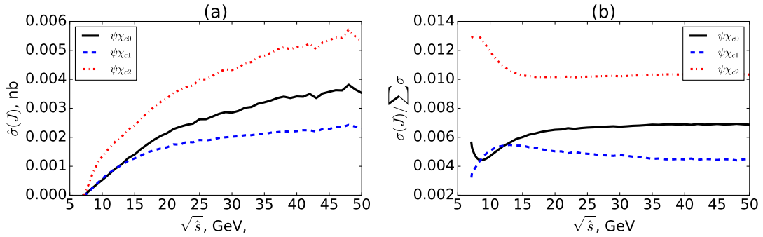
Figure 3. Partonic cross sections of J/\psi\chi_{cJ} reactions
