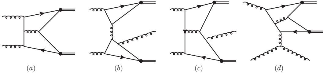
Figure 1. Typical Feynman diagrams of double charmonium production in gluon interaction at LO (a) and NLO* (b,c,d)
