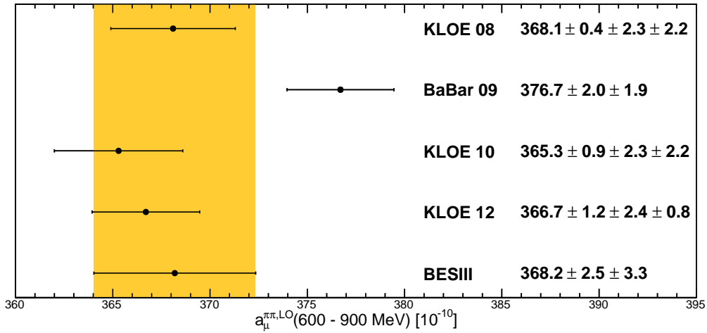
Figure 4. Comparison of a_{\mu}^{\pi\pi, LO}(600 - 900\text{MeV}) from the measurements of KLOE, BaBar, and BESIII. The error bars include statistical and systematical errors. Figure is taken from Ref. [17].
