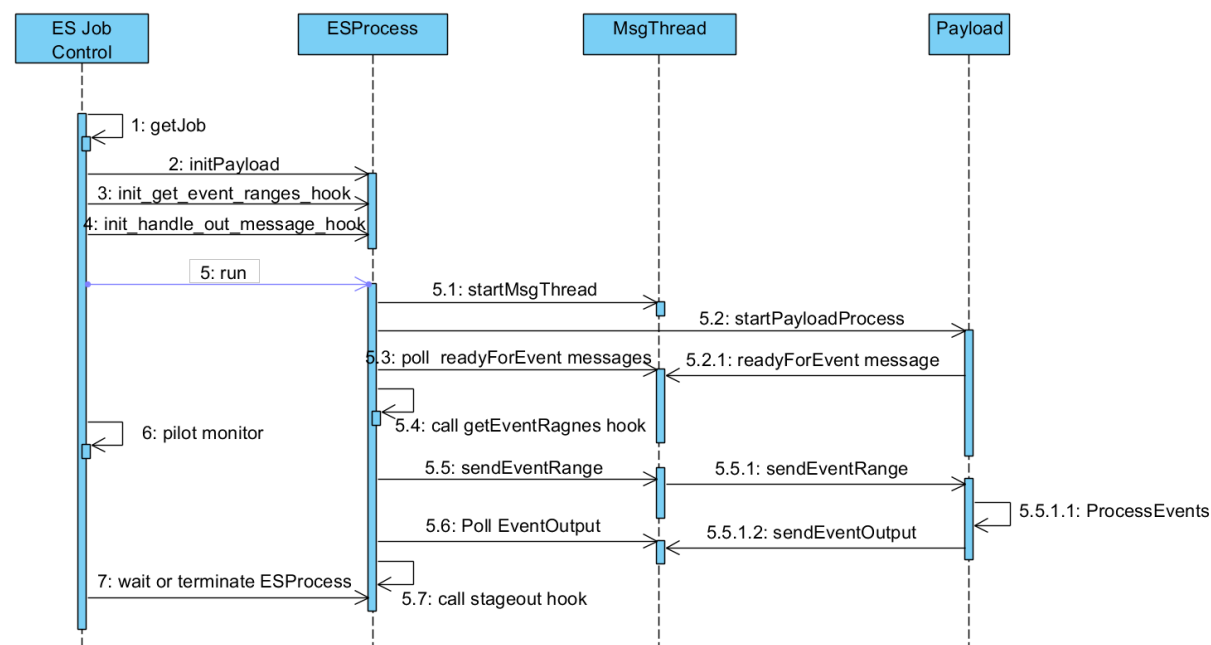
Figure 3. Sequence diagram for the Event Service workflow as used in ATLAS.
