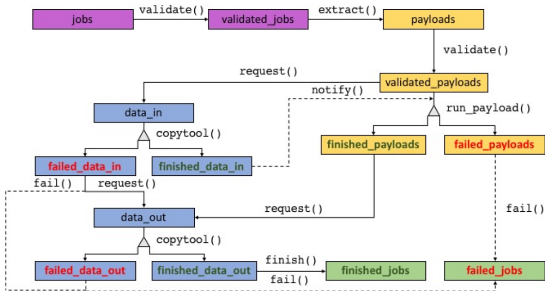
Figure 2. The generic flow of the job objects.
