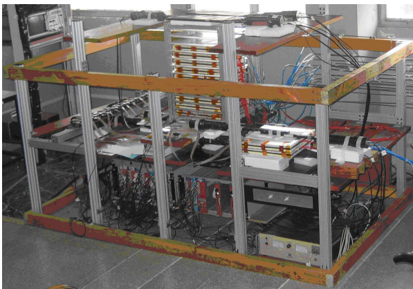
(a) Cosmic ray muon telescope
