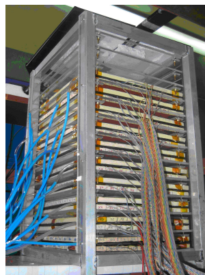
(b) Stack of tracking RPCs
