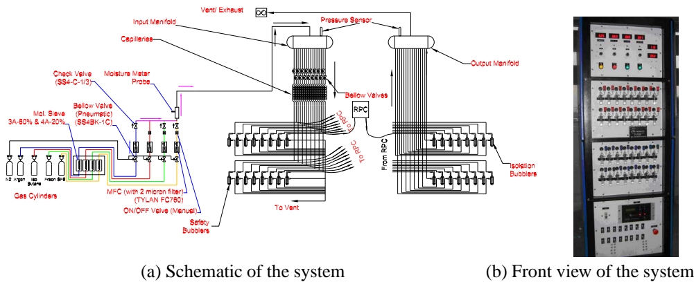
Figure 3. New gas mixing and distribution system
