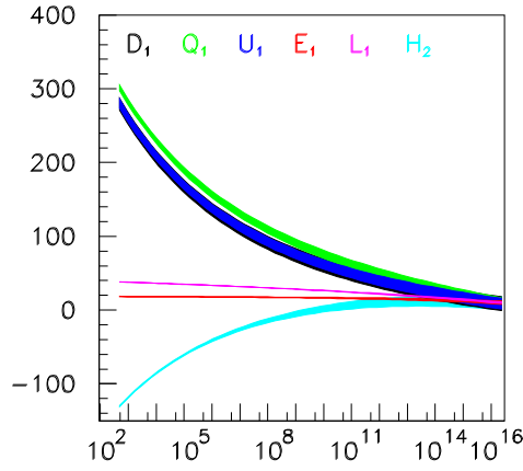
Figure 3. Evolution of scalar quark and lepton and Higgs mass parameters in an minimal supergravity point using inputs from expected results in LHC and ILC combined analysis. From Ref. [34].
