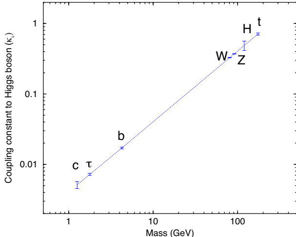
Figure 1. Precision of the coupling-constant determination at ILC with \mathcal{L} = 500 \text{ fb}^{-1} . The coupling constant \kappa_i is defined from the Higgs boson coupling to the “ i ” particle. m_i = \kappa_i v holds in the Standard Model. The Higgs boson mass is taken to be 120 GeV. For the charm, tau, bottom, W and Z coupling measurements, \sqrt{s} = 300 \text{ GeV} is assumed. \sqrt{s} = 500 \text{ GeV} (700 GeV) is taken for the Higgs self-coupling ( t\bar{t}H ) coupling measurement. From Ref. [4].
