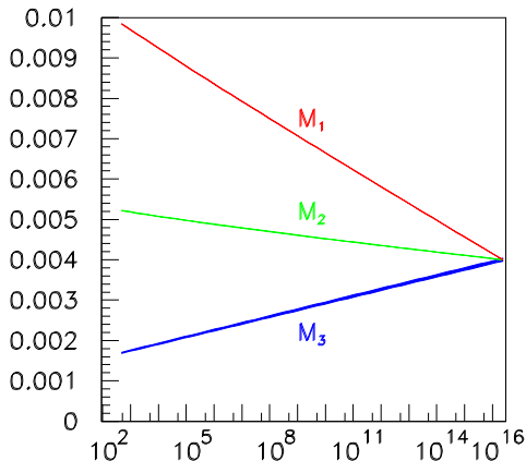
Figure 2. Evolution of three gaugino masses parameters in the SUSY GUT using inputs from LHC and ILC measurements. From Ref. [34].
