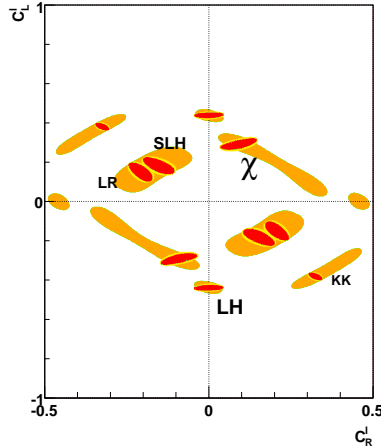
Figure 4. Resolving power (95% CL) for M_{Z'} = 2 TeV and \sqrt{s} = 500 GeV, \mathcal{L}_{int} = 1\text{ab}^{-1} for leptonic couplings based on the leptonic observables \sigma_{P_{e^-}P_{e^+}}^\mu , A_{LR}^\mu , and A_{FB}^\mu . The largest region corresponds to the unpolarized case while the smallest region corresponds to electron and positron polarization of 80% and 60% respectively with the middle region corresponding to only electron polarization. The couplings correspond to various models with a Z' boson ( E_6 , \chi , LR, LH, SLH and KK models). From Ref. [42].
