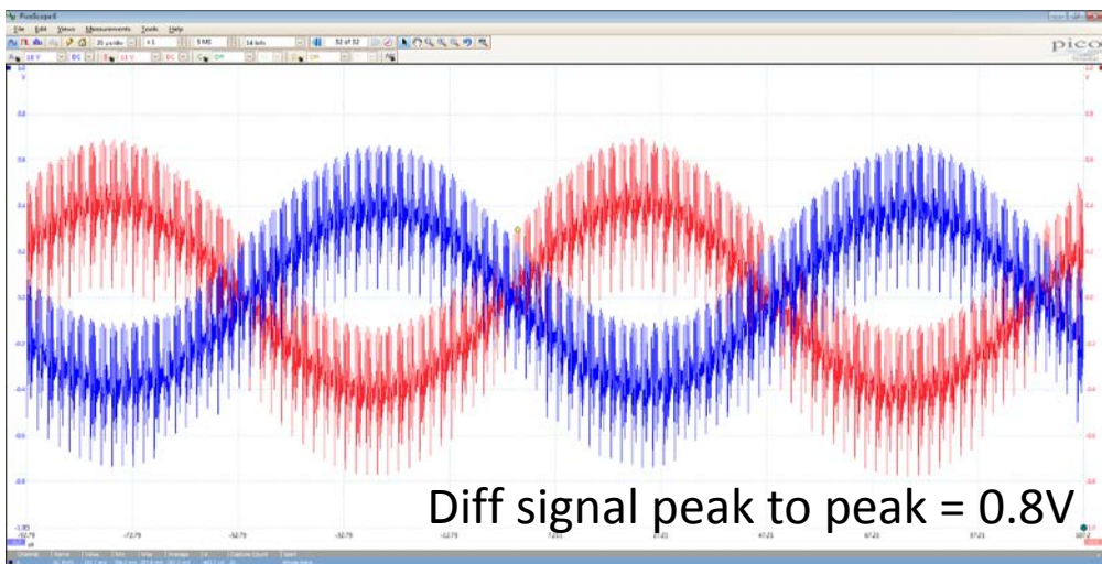
PSB prototype 2, Rotasyn RO5032-452, SN.9026
