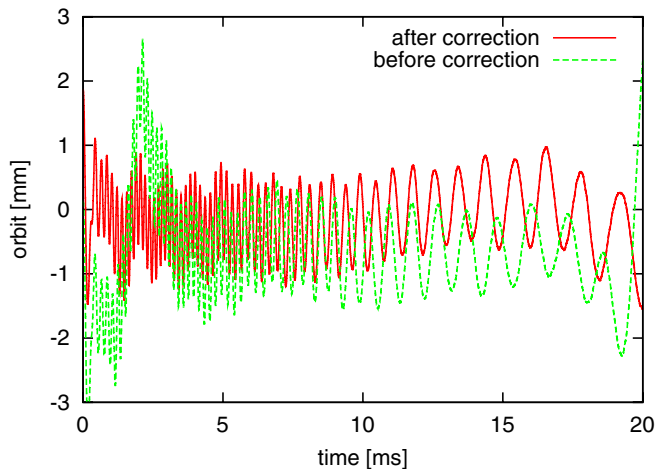
FIG. 18. (Color) Horizontal beam position data on \Delta R -BPM over the acceleration process (20 ms) before (dashed green curve) and after (solid red curve) the rf frequency tuning.
