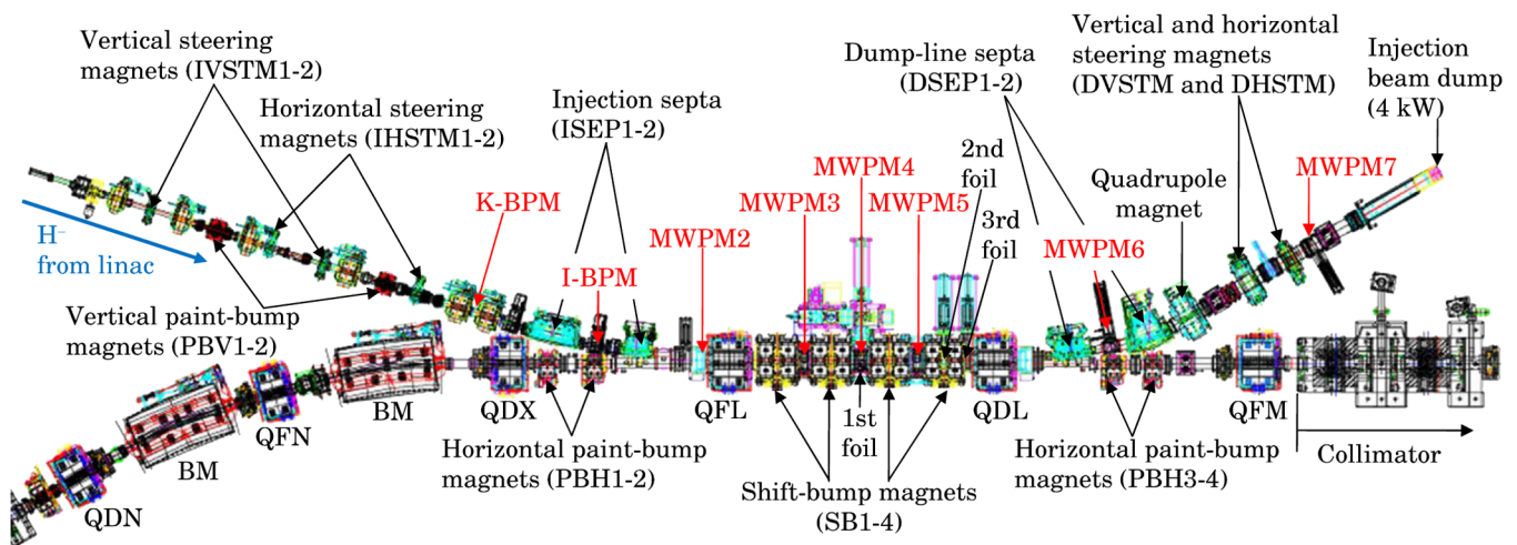
FIG. 2. (Color) Schematic view of the RCS injection area, where the red characters correspond to the beam diagnostics devices defined in Table II.
