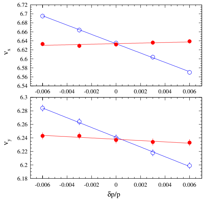
FIG. 9. (Color) Horizontal (upper) and vertical (lower) betatron tunes as a function of the momentum offset measured in the beam storage mode before (open blue circles) and after (closed red circles) the chromaticity correction.
