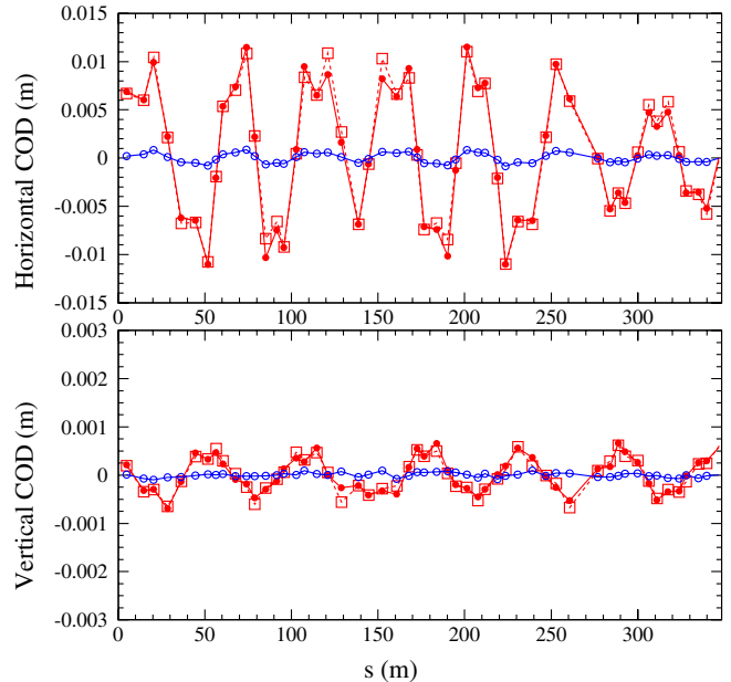
FIG. 13. (Color) Horizontal (upper) and vertical (lower) COD caused by the leakage field from ESEP excited at 181 MeV (open blue circles) or at 3 GeV (closed red circles) measured in the 181 MeV beam storage mode, in which open red squares show the COD obtained in the model fitting for the closed red circle data.
