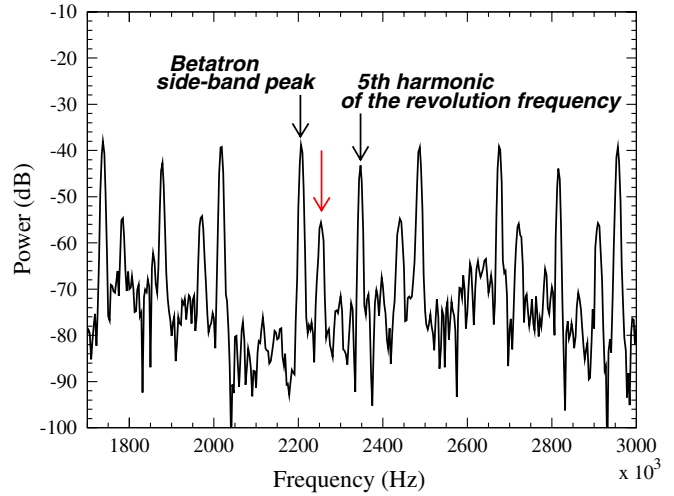
FIG. 16. (Color) FFT spectrum for horizontal BPM data taken for 0.16 ms time span with 6.4 MHz sampling in the middle of the injection process. As for the red arrow, see the text.
