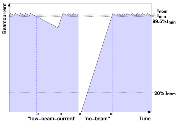
Figure 1: A “no-beam” failure starts when the beam current drops below 20% of the nominal beam current I_{nom} ; a “low-beam-current” already below 99.5% of the nominal lower current limit I_{min} (if it isn’t a “no-beam” failure). Both modes stops when the nominal beam current I_{nom} is reached again.
