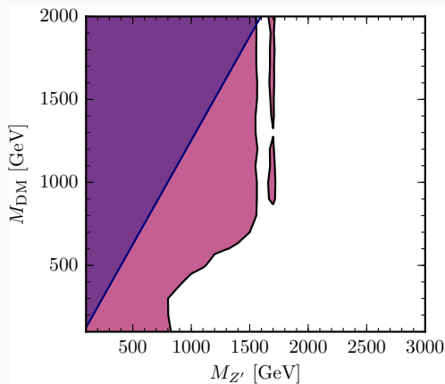
(c) g_q = 0.375 and g_{DM} = 1
