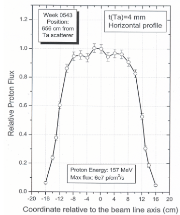
Figure 10: TSL Uppsala beam profile
