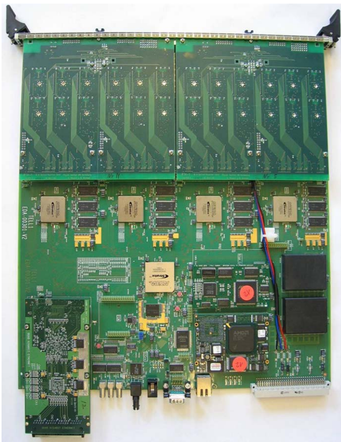
Figure 8: TELL1 DAQ Board (Lausanne)
