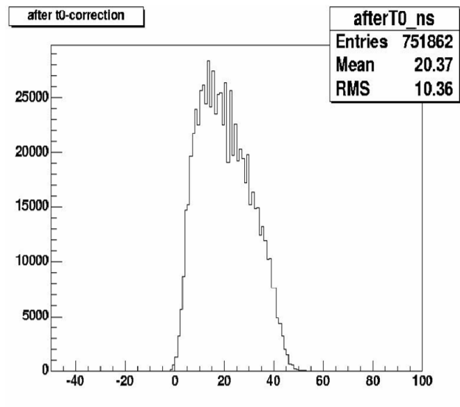
Figure 9: Drift Times t_0 corrected
