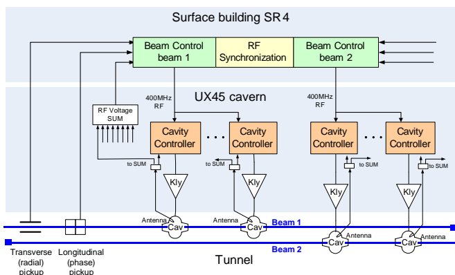
Figure 2: 400 MHz Low-Level system layout (simplified)
