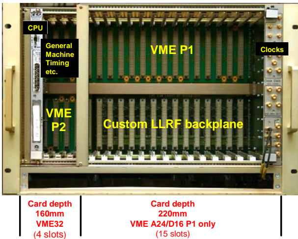
Figure 4: Custom LLRF VME crate
