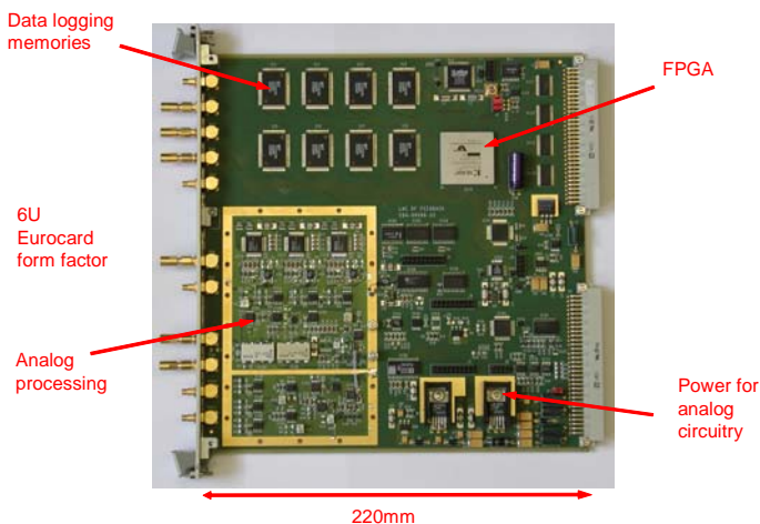
Figure 3: Typical RF Low-Level module: RF feedback
