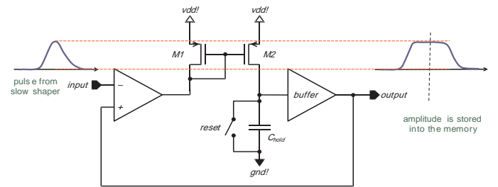
Figure 11: Block schematic of the peak-detector and hold circuit.
