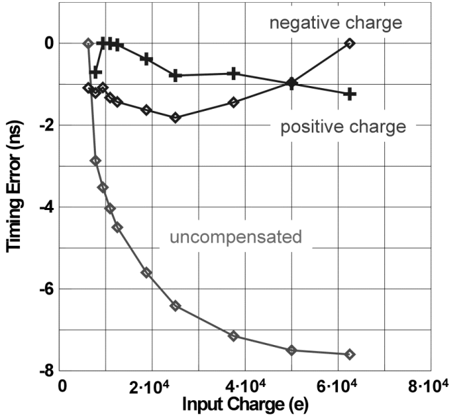
Figure 8: Measured time walk after the discriminator and time walk compensation circuits: The timing error is reduced to \leq 2 ns (results from the DETN1FE10 test chip [3]).
