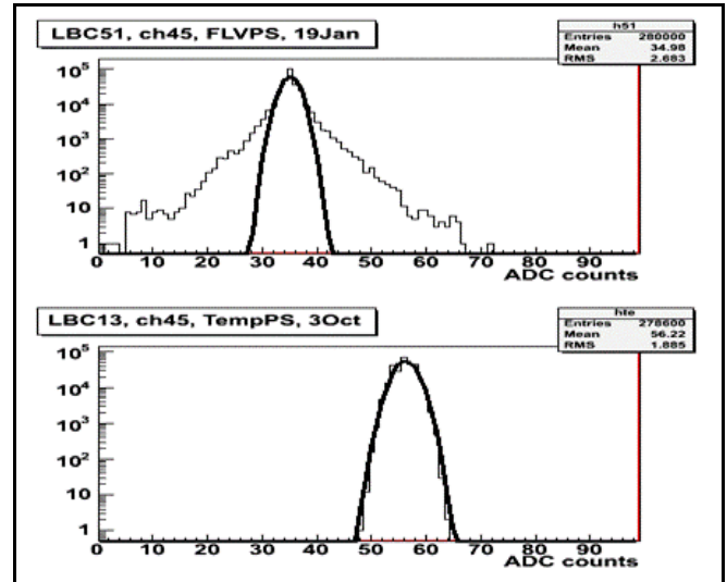
Figure 7: non Gaussian distribution of pedestals when using the unfiltered finger power supply (top) versus Gaussian distribution when using a commercial power supply (bottom).
