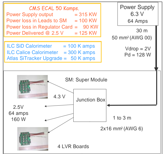
Figure 1: ECAL Power Distribution
