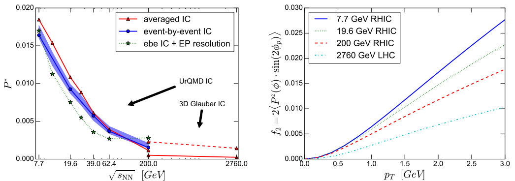
Figure 1. Left panel: collision energy dependence of global \Lambda polarization along global angular momentum of the fireball, calculated with averaged initial state from UrQMD ( \sqrt{s_{\text{NN}}}=7.7, \dots, 200 GeV) and Monte Carlo Glauber ( \sqrt{s_{\text{NN}}}=200, 2760 GeV). Right panel: second order Fourier harmonic coefficient of polarization component along beam direction, calculated as a function of p_T for different collision energies; 200 and 2760 GeV points correspond to Monte Carlo Glauber initial state.
