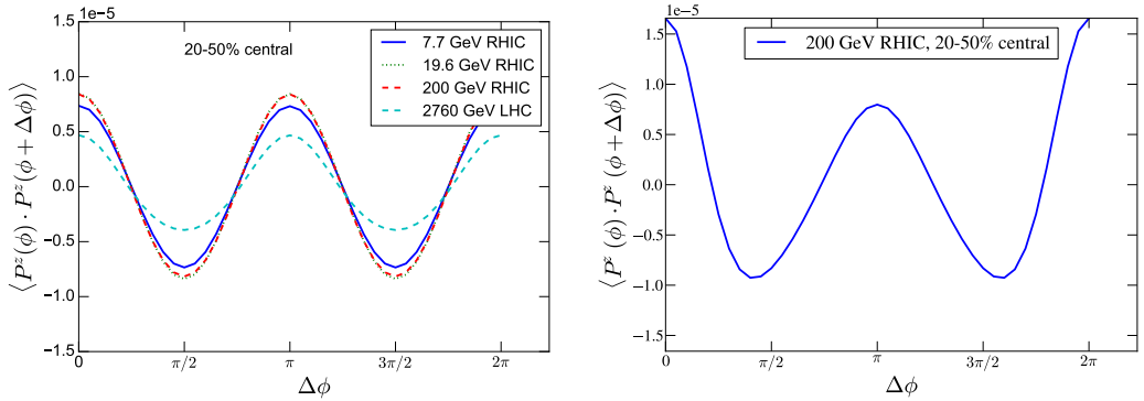
Figure 2. Covariance of polarization components in beam direction, for pairs of midrapidity \Lambda separated by azimuthal angle \Delta\phi in transverse momentum space. Left panel: results with averaged initial state from UrQMD ( \sqrt{s_{NN}}=7.7, \dots, 200 GeV Au-Au) and Monte Carlo Glauber ( \sqrt{s_{NN}}=200 Au-Au, 2760 GeV Pb-Pb). Right panel: event-by-event hydrodynamic calculation with UrQMD initial state for Au-Au collisions at \sqrt{s_{NN}} = 200 GeV.
