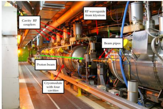
Figure 2.2: LHC cavity module in machine tunnel [2]
