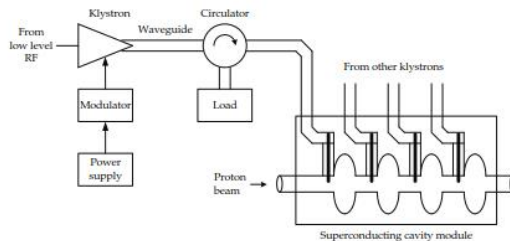
Figure 2.3: The acceleration RF systems in the LHC
