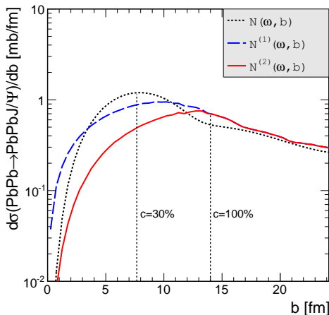
Figure: Differential cross section for photoproduction of J/\psi meson as a function of impact parameter for \sqrt{s_{NN}} = 2.76 \text{ TeV} . Different lines correspond to different approximations: dotted - standard UPC approach (Eq. (11)), dashed - first approximation/correction (Eq. (14)) (upper limit), solid - second approximation/correction (Eq. (15)) (lower limit). Here
