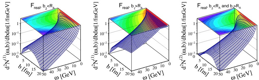
Figure: Two-dimensional distributions of the photon fluxes N^{(1)}(\omega, b) (see Eq. (14)) and N^{(2)}(\omega, b) (see Eq. (15)) in the impact parameter b and in the energy of photon \omega for three different conditions (more in the text).
