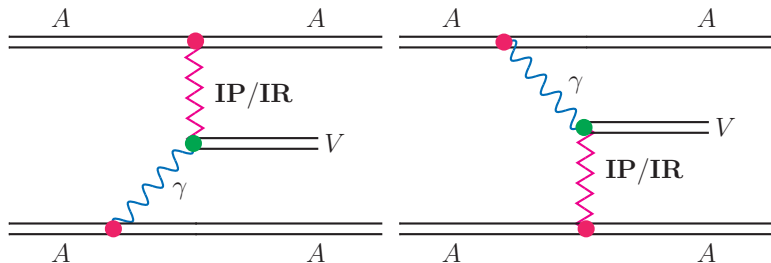
Figure: Schematic diagrams for the single vector meson production by photoproduction (photon- \mathbf{P}/\mathbf{R} (left) or \mathbf{P}/\mathbf{R} -photon (right) fusion). Here the symbol \mathbf{P}/\mathbf{R} is an abbreviation for multiple diffractive scattering of the hadronic system in the nuclear medium.
