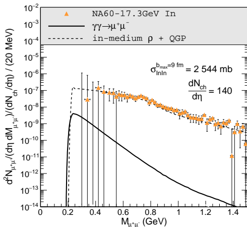
Figure: Low- P_T ( <0.2 GeV) acceptance-corrected dimuon invariant mass excess spectra in the rapidity range 3.3 < Y_{\mu^+\mu^-, \text{LAB}} < 4.2 for MB In+In ( \sqrt{s_{NN}}=17.3 GeV) collisions at the SPS. Calculations for coherent \gamma\gamma fusion (solid line) and thermal radiation (dashed line) are compared to NA60 data.
