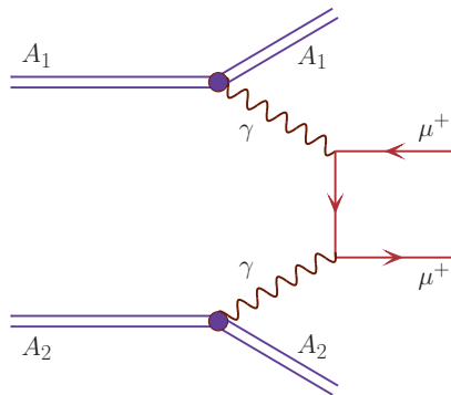
Figure: Mechanism of production of lepton pairs.
