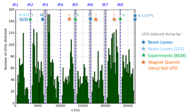
Figure 3: UFO's leading to premature beam dumps by subsequent losses during 2016 operation..
