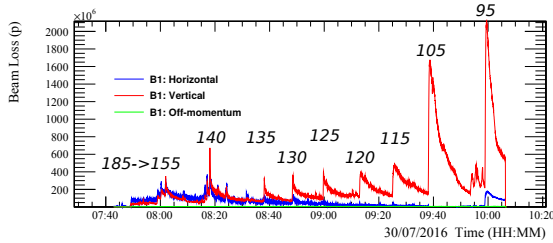
(c) Losses
