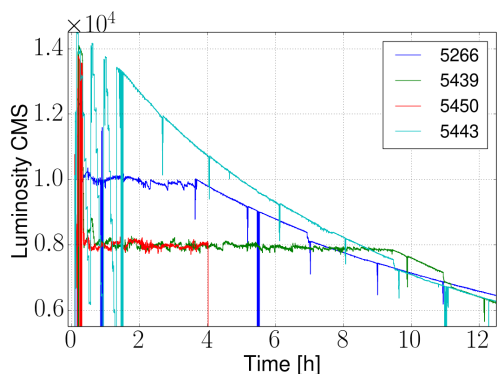
(a) Instantaneous luminosity
