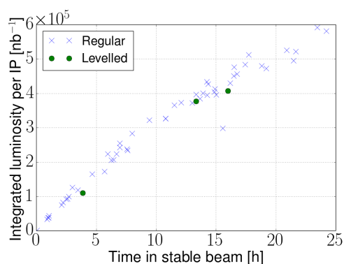
(b) Integrated luminosity
