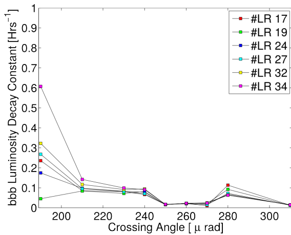
(c) Luminosity
