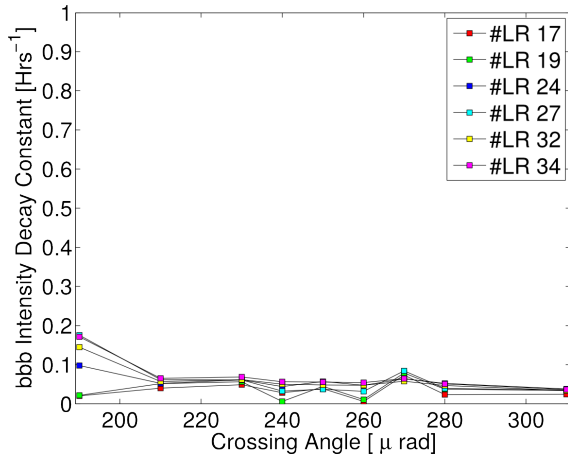
(b) Beam 2
