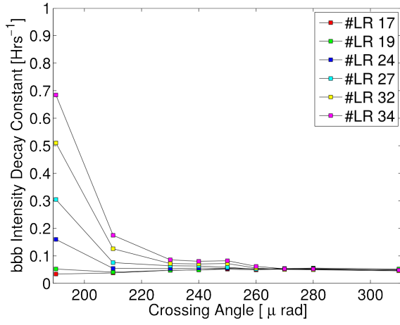
(a) Beam 1
