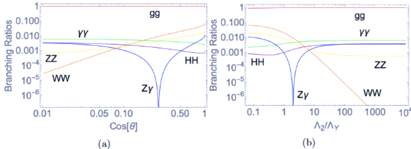
Figure 5: Branching ratios of the scalar resonance decaying into the gauge boson pairs and the Higgs boson pair as functions of \cos\theta [plot (a)] and \Lambda_2/\Lambda_Y [plot (b)] for M_S = 750 GeV, and \Lambda_H = 4 TeV. (a) and (b) are depicted for \lambda = 0.01 .
