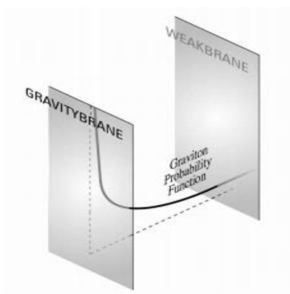
Figure 2.1: Schematic view of Randall-Sundrum model where the graviton is the only particle propagating in the extra dimension.
