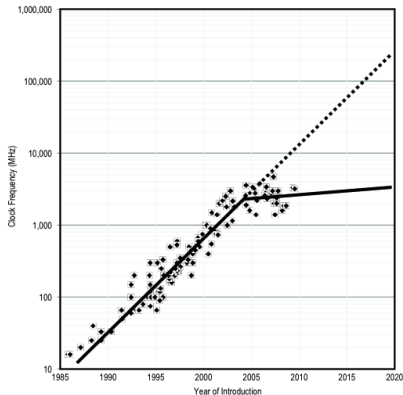
Clock Frequency vs Time
