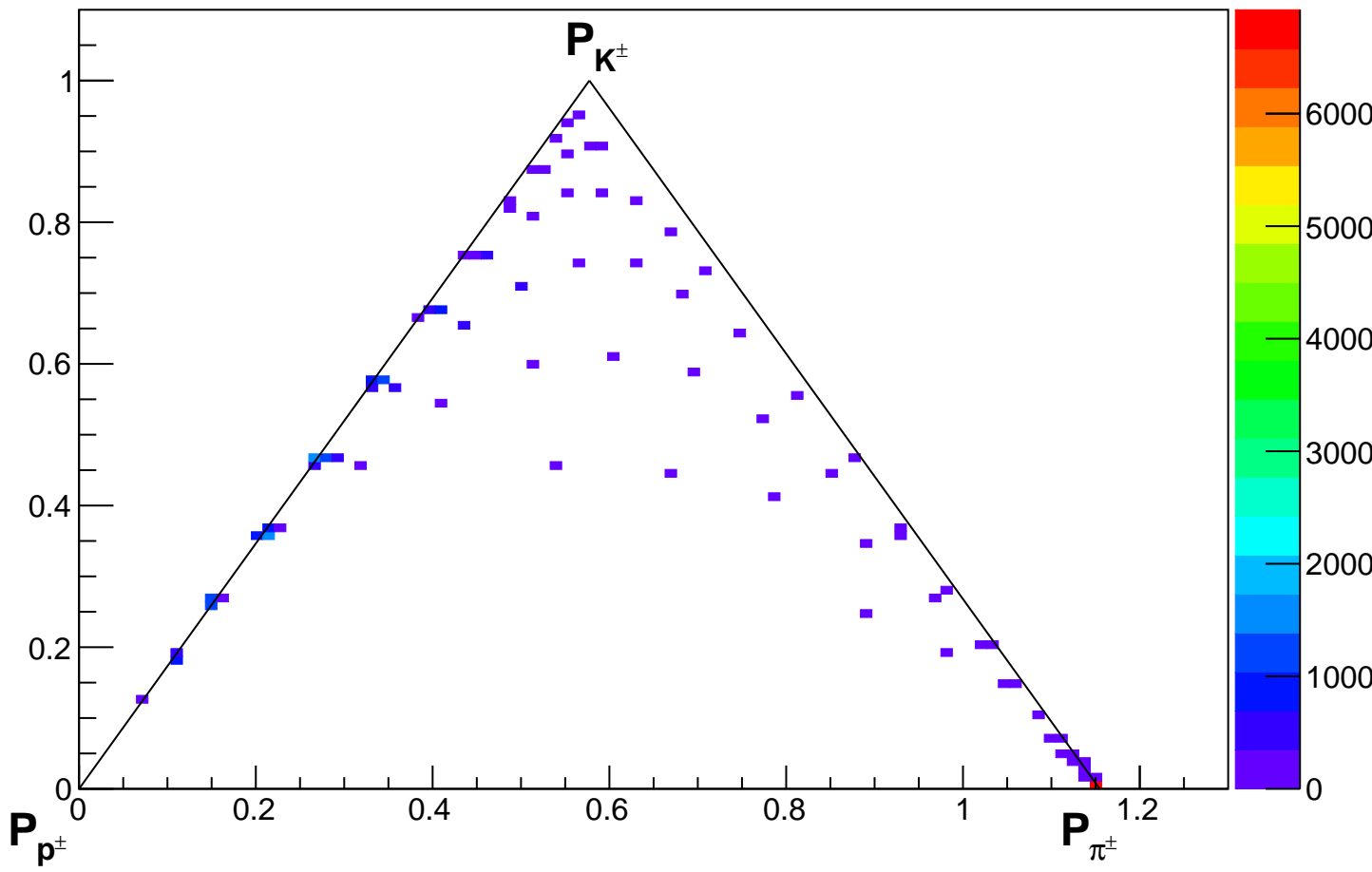
Separation triangle, E = 2.0 TeV, Detectors 1 and 2
