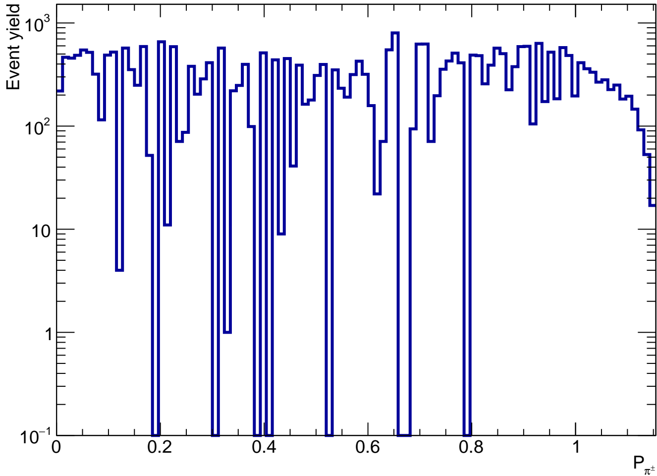
Projection over the P_{\text{IK}} axis in Detectors 1 and 3, E = 1.0 TeV
