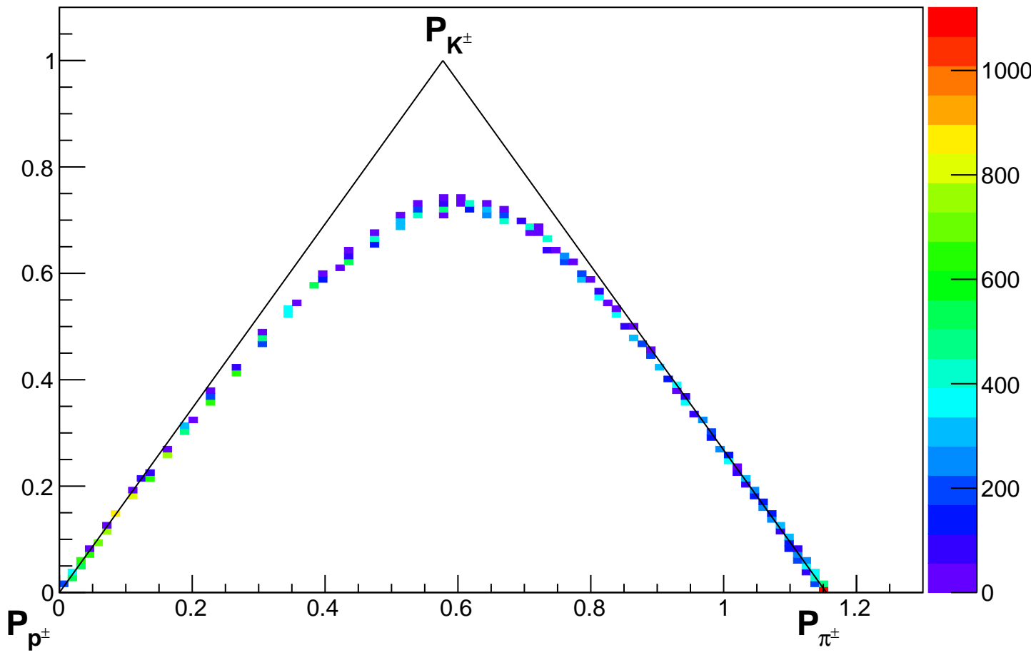
Separation triangle, E = 4.0 TeV, Detectors 1 and 2
