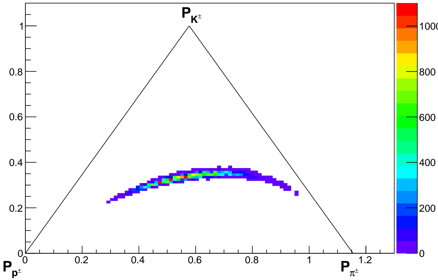
Separation triangle, E = 6.0 TeV, Detectors 1 and 3
