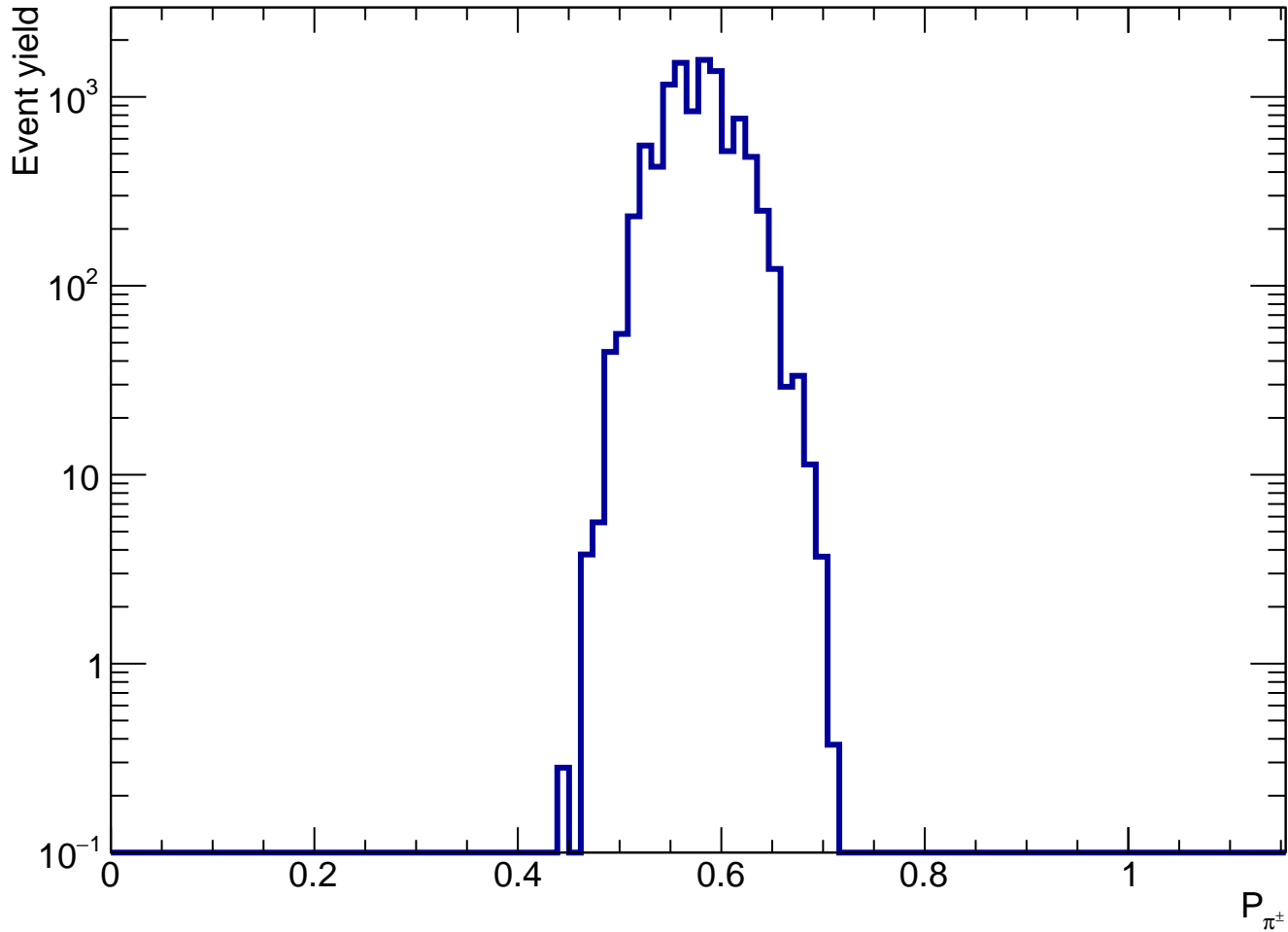
Projection over the P_{\pi^\pm} axis in Detector 2, E = 1.0 TeV
