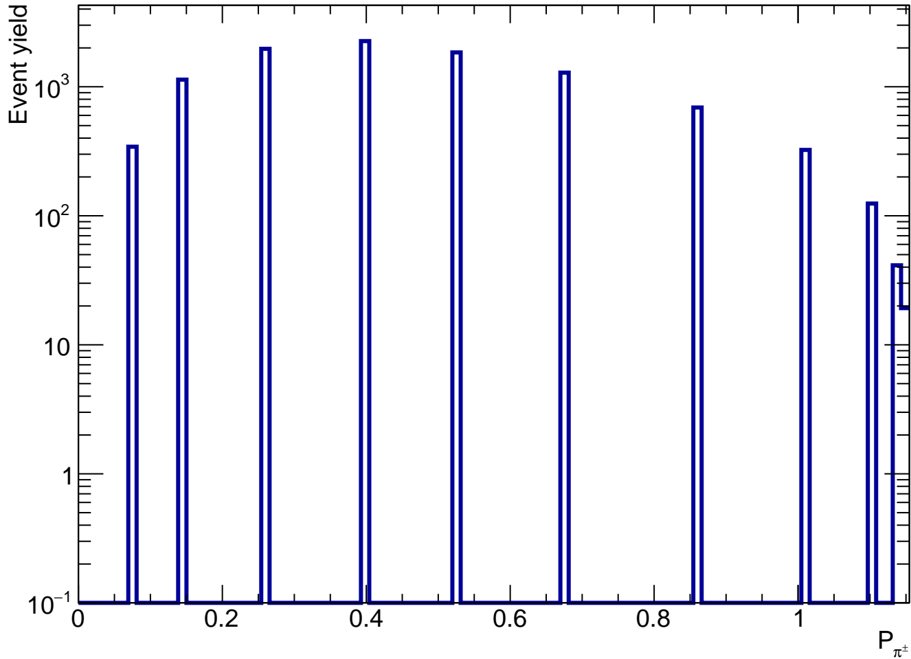
Projection over the P_{\pi^\pm} axis in Detector 1, E = 1.0 TeV
