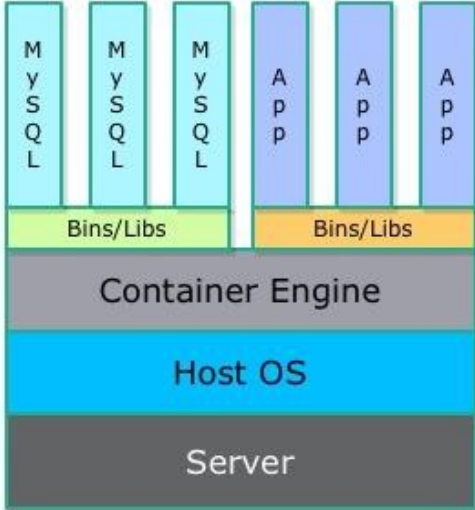
Containers
