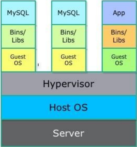
Virtual Machines
