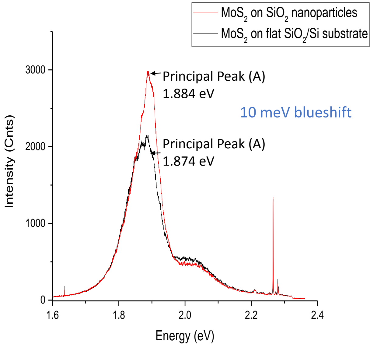
Photoluminescence Emission Spectra of Monolayer MoS 2
