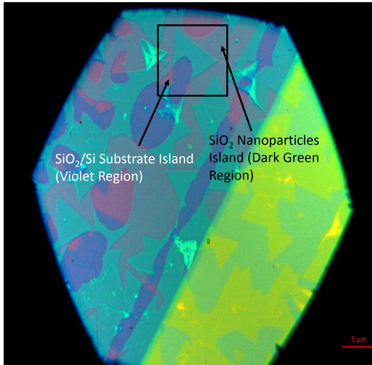
Optical Image of Monolayer MoS 2 Flakes on SiO 2 /Si Substrate and SiO 2 Nanoparticles
