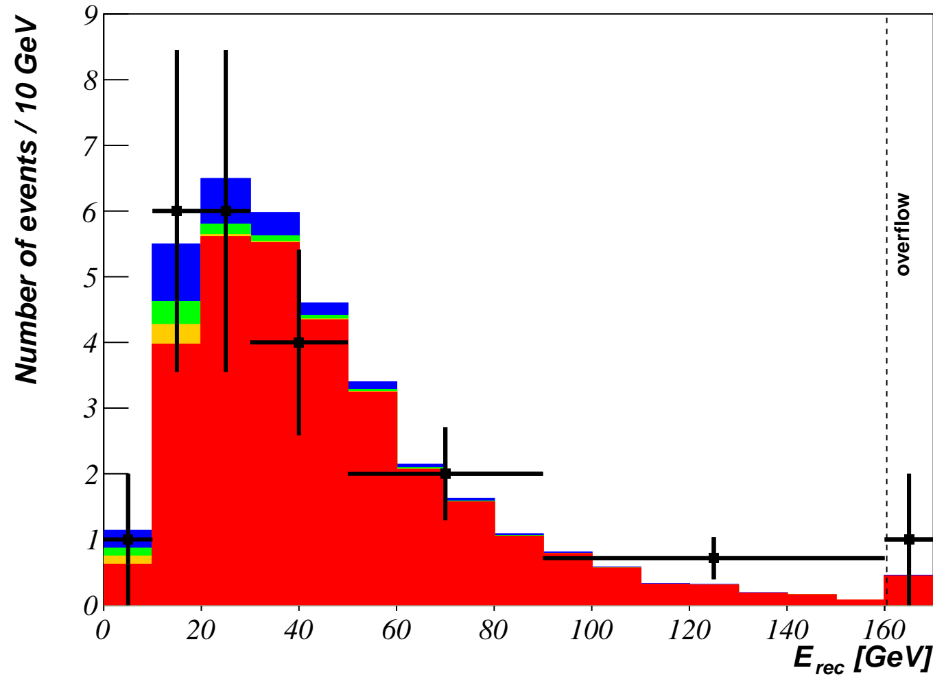
Energy spectrum of \nu_e candidates (2008-2012 data)
