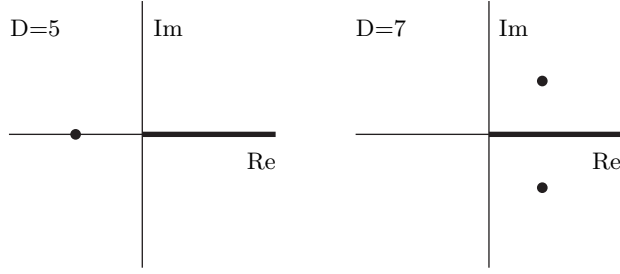
Fig. 2. The analytical structure of the gauge field propagator
