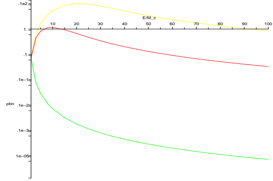
Fig. 4. The differential cross section for eq \rightarrow eq scattering
