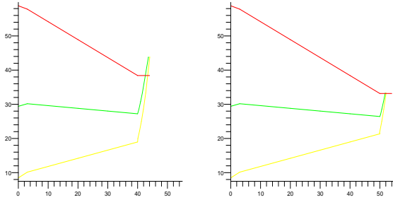
Fig. 6. The running of the coupling constants in the MSSM
