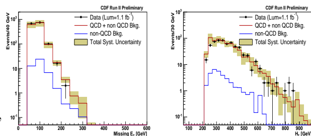
Fig. 1. E_T and H_T in QCD-dominated samples, after all selection cuts for the 4-jet region: data are superimposed to QCD+non-QCD background with total systematics uncertainties. All cuts have been applied except the one on the variable that is represented.
